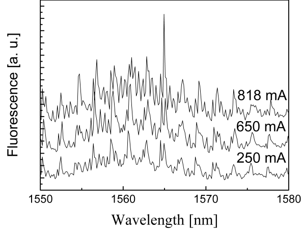
Fig. 28. – Fluorescence spectra measured for a 250 \mu\text{m} microsphere coated by a 70SiO 2 - 30HfO 2 film of 0.8 \mu\text{m} in thickness, activated by 1 mol% Er 3+ for different values of the exciting pump power. In the figure are indicated the values of the exciting laser current [131].
