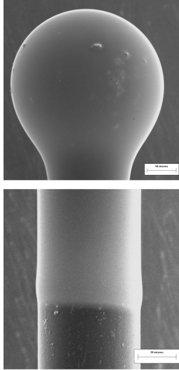
Fig. 25. – SEM image of 1% mol \text{Er}^{3+} activated 70\text{SiO}_2 - 30\text{HfO}_2 films deposited on a silica microsphere using the sol-gel method (above) and the SEM image of the coated fiber on top of which the microsphere is located (below). The bar in the two photos is 50\text{ }\mu\text{m} . [132].
