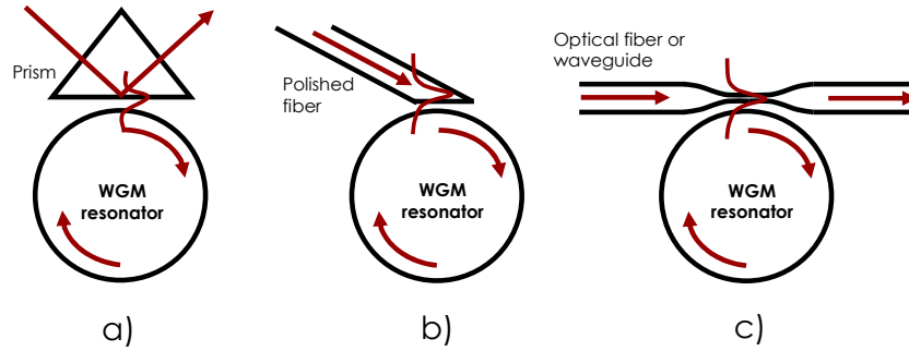
Fig. 9. – a) Prism coupling using frustrated total internal reflection. b) Slant-cut optical fiber coupling. c) Tapered fiber or optical waveguide coupling.
