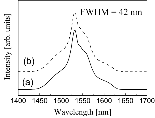
Fig. 26. – Photoluminescence spectra relative to the {}^4I_{13/2} \rightarrow {}^4I_{15/2} transition of the \text{Er}^{3+} ions for: 0.3 mol% \text{Er}^{3+} activated 70\text{SiO}_2 -30 \text{HfO}_2 coated silica microsphere (a) and planar waveguide (b) obtained using the sol-gel method. Spectra were obtained upon excitation at 980 nm. [132].
