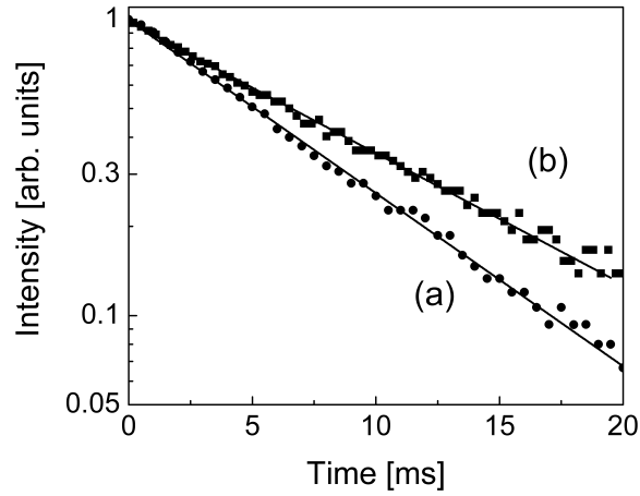
Fig. 30. – Decay curves of the luminescence from the ^4I_{13/2} metastable state of \text{Er}^{3+} ions for (a) 70\text{SiO}_2\text{-}30\text{HfO}_2 glass-ceramic planar waveguide activated by 0.3 mol% \text{Er}^{3+} ; (b) glass-ceramic spherical microresonator coated by a film of 70\text{SiO}_2\text{-}30\text{HfO}_2 activated by 0.3 mol% \text{Er}^{3+} [134].
