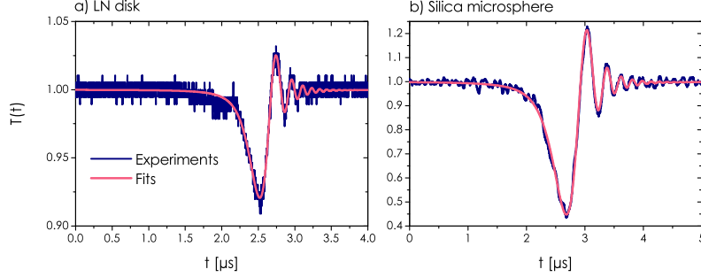
Fig. 13. – Experimental transient profile of the transmission T(t) a) for the LN disk and b) for the silica microsphere. We also represent the numerical fit from which we infer the values of \tau_0 , \tau_e and \hat{V}_S .
