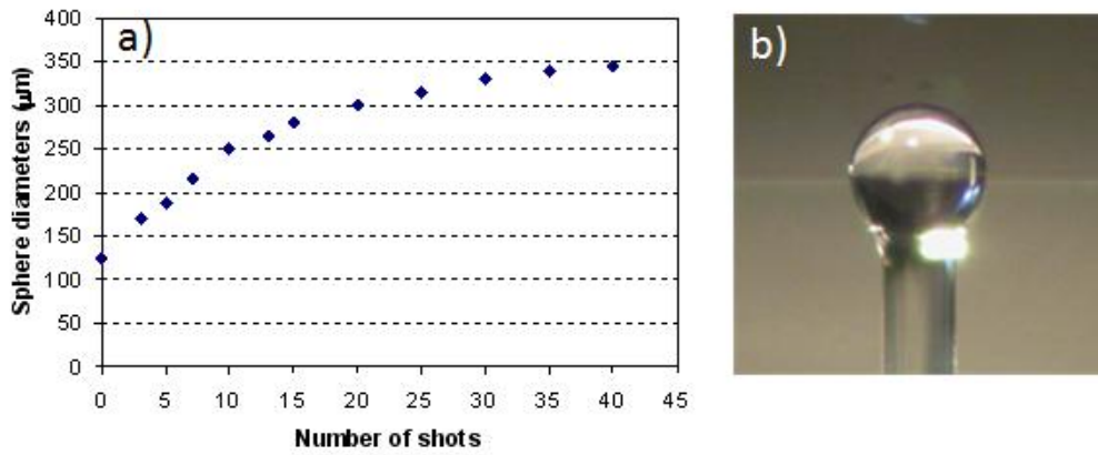
Fig. 20. – a) Size of the microspheres produced at the tip of a standard 125 \mu\text{m} telecom fiber, as a function of the arc shots in a fiber fusion splicer. b) Optical image of a microsphere with a diameter of about 250 \mu\text{m} . In the background (out of focus) one can see the coupling tapered fiber. [120]
