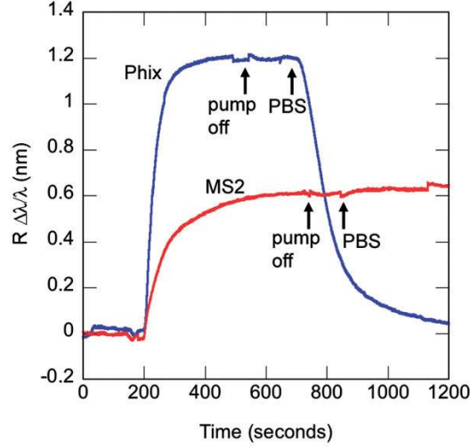
Fig. 38. – Comparison between Phix174 (blue line) and MS2 (red line) experiments on the same sphere. (Reproduced by permission of The Royal Society of Chemistry. [167])
