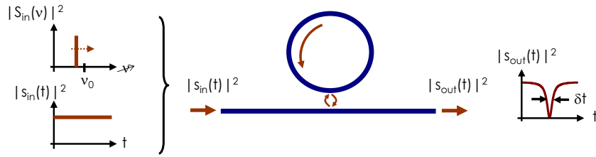
Fig. 10. – Schematic view of the Q-factor measurement method.
