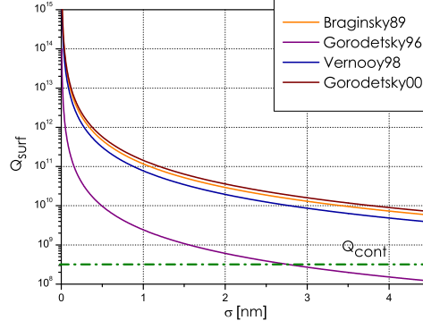
Fig. 5. – Comparison of the evolution of Q_{s.s} vs \sigma given by: Eq.(22) noted Braginsky89, Eq.(23) noted Gorodetsky96, Eq.(24) noted Vernoooy98 and Eq.(25) noted Gorodetsky00 with B = 5 \text{ nm} and D = 100 \mu\text{m} . (From S. Trebaol PhD thesis [68].
