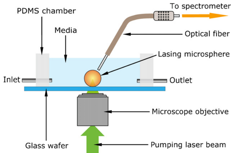
Fig. 19. – Experimental setup for microsphere excitation and laser output observation. The open chamber is obtained by bonding a PDMS frame ( 10\text{mm} \times 20\text{mm} in size and 3\text{mm} in height) to a glass wafer. The pulse width of the pumping laser was less than 10 \text{ ns} and the frequency was 20 \text{ Hz} . (Reproduced with permission from [113].)
