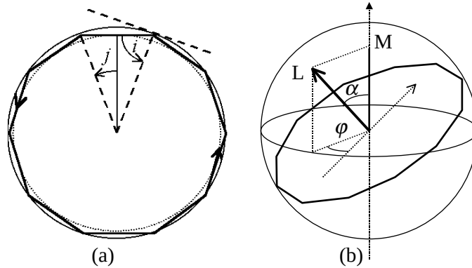
Fig. 1. – (a) Ray of light propagation by TIR in spherical cavity. (b) Angular momentum L associated with WGM and its M projection on polar axis.
