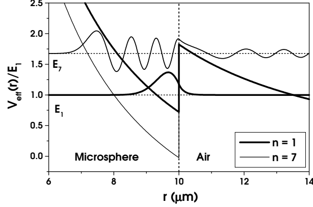
Fig. 2. – Effective potential and radial functions associated with, for an equivalent particle and turning point for fundamental energy E_1 ( n = 1 ) and E_7 ( n = 7 ) in the case of a TE mode ( \ell = 100 ) in a silica microsphere ( a = 10 \mu m , N = 1.45 )
