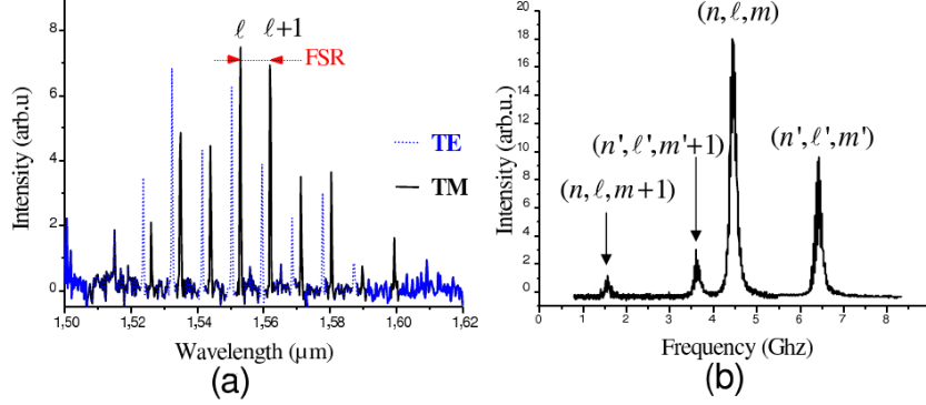
Fig. 4. – (a) WGM fluorescence spectrum of Er:ZBLAN microsphere coupled by prism (b) fine structure of the TM peak at 1.562 \mu m
