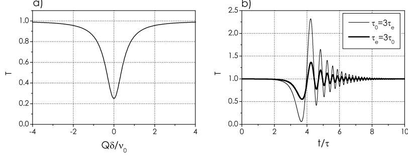
Fig. 11. – a) Stationary transmission profile for a resonator in the undercoupling ( \tau_e = 3\tau_0 ) and overcoupling ( \tau_0 = 3\tau_e ) regimes, the two curves are superimposed. b) Transmission in the dynamic case with a frequency sweeping rate: \tilde{V}_S = 2.25\tilde{V}_0 .
