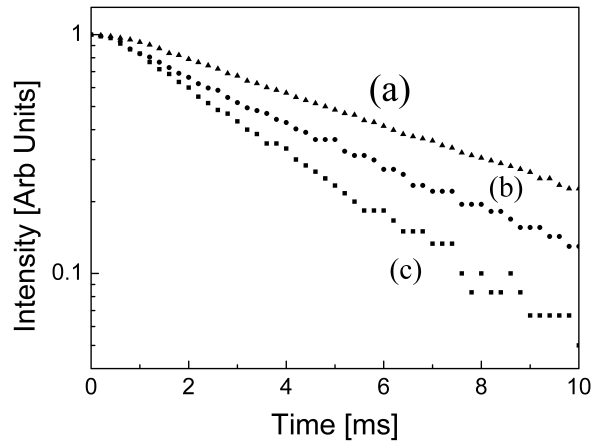
Fig. 27. – Decay curves of the {}^4I_{13/2} metastable state of \text{Er}^{3+} ions in the 70\text{SiO}_2 -30 \text{HfO}_2 coated microspheres activated by (a) 0.3 mol% \text{Er}^{3+} (b) 0.5 mol% \text{Er}^{3+} and (c) 1 mol% \text{Er}^{3+} [132].
