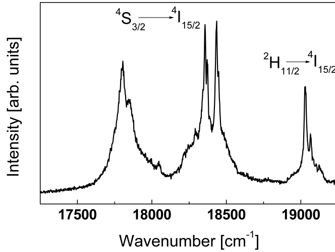
Fig. 31. – Room temperature luminescence spectra of the ^4S_{3/2} \rightarrow ^4I_{15/2} and ^2H_{11/2} \rightarrow ^4I_{15/2} transitions of \text{Er}^{3+} ion for a 100\text{ }\mu\text{m} glass-ceramic microsphere coated with 70\text{SiO}_2\text{-}30\text{HfO}_2 layer [134].
