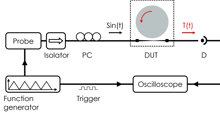
Fig. 12. – Q-factor measurement experimental setup. The probe laser is a tunable narrow linewidth (150 – 300kHz) laser. PC is a polarizer controller, D is a photodetector. The DUT (device under test) is either a LN microdisk coupled using a LN waveguide or a silica microsphere coupled using a tapered fiber.
