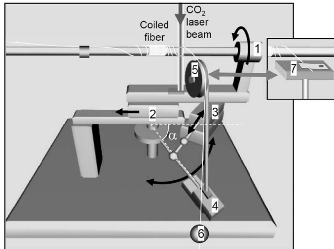
Fig. 14. – Sketch of the experimental setup for fiber coil fabrication: 1 a rotary gear motor; 2, 3, 4 translation stages; 5 a wheel supporting the incoming fiber; 6 a weight; 7 a fiber clamp. (Reproduced with permission from [101].)
